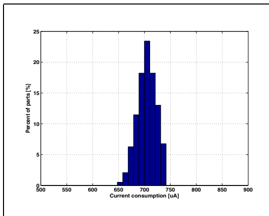
Figure 17. Current consumption in normal mode at 3.3 V
